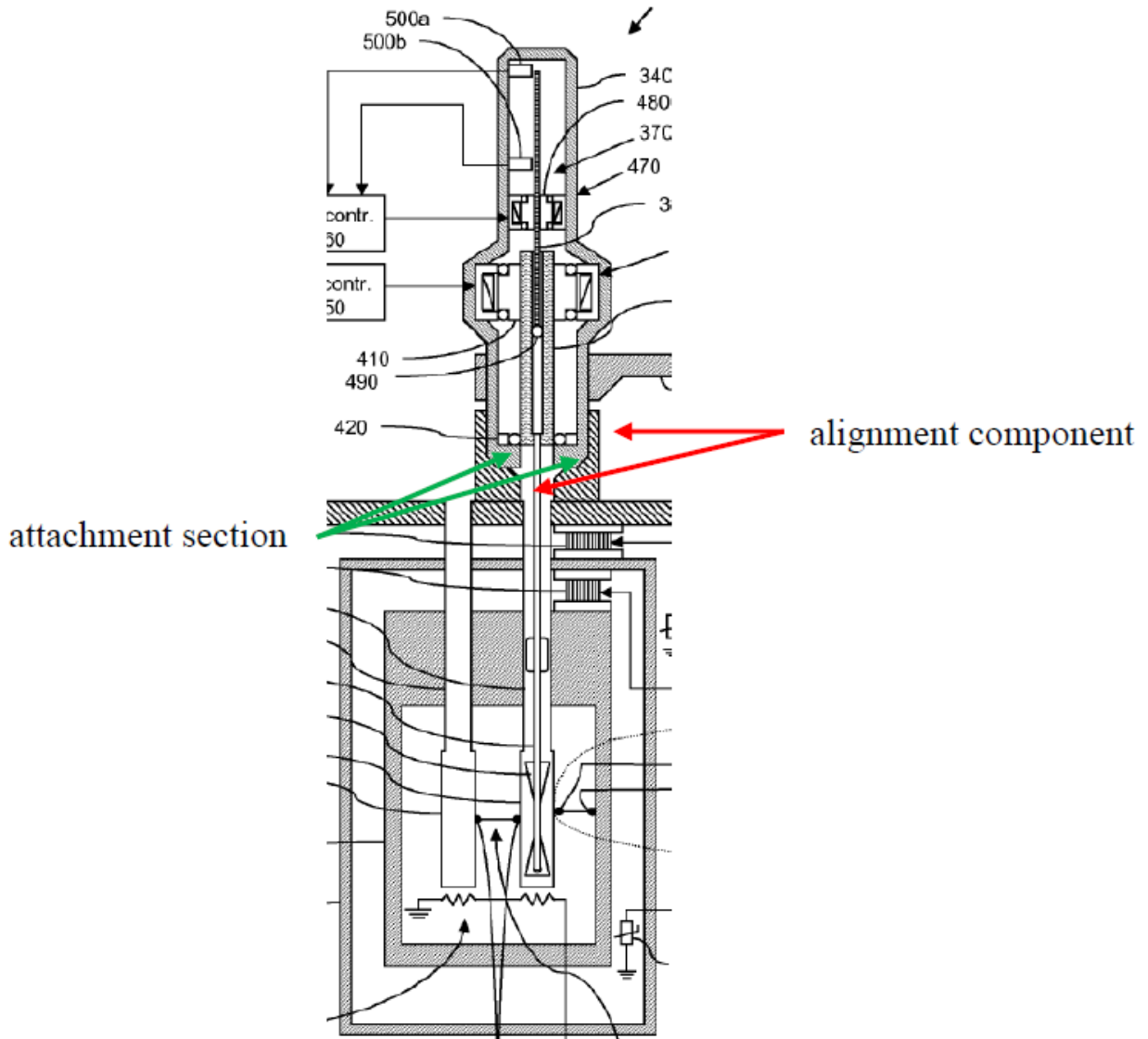
'549 Patent at Fig. 2 (annotated and cropped)
