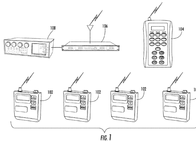
Figure 1 depicts recording system 100, which “wirelessly records audio events, such as performances, movie takes, etc. having one or more
